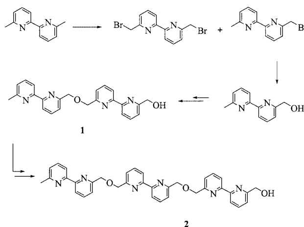
Scheme 1. Synthesis of poly(bipyridines) 1 and 2
